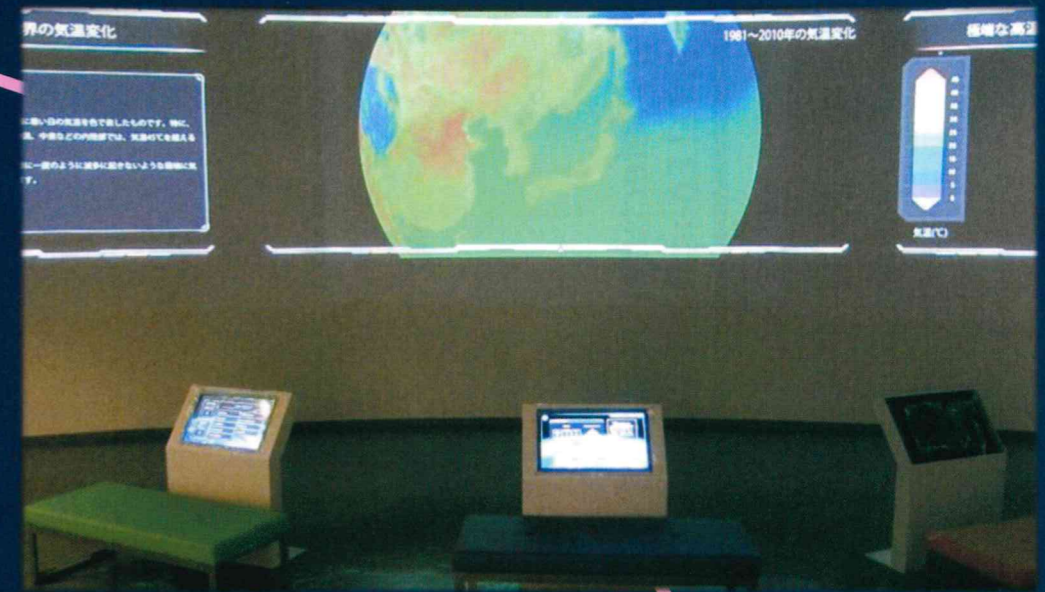
② Simulation on How Global Warming Changes the Climate
